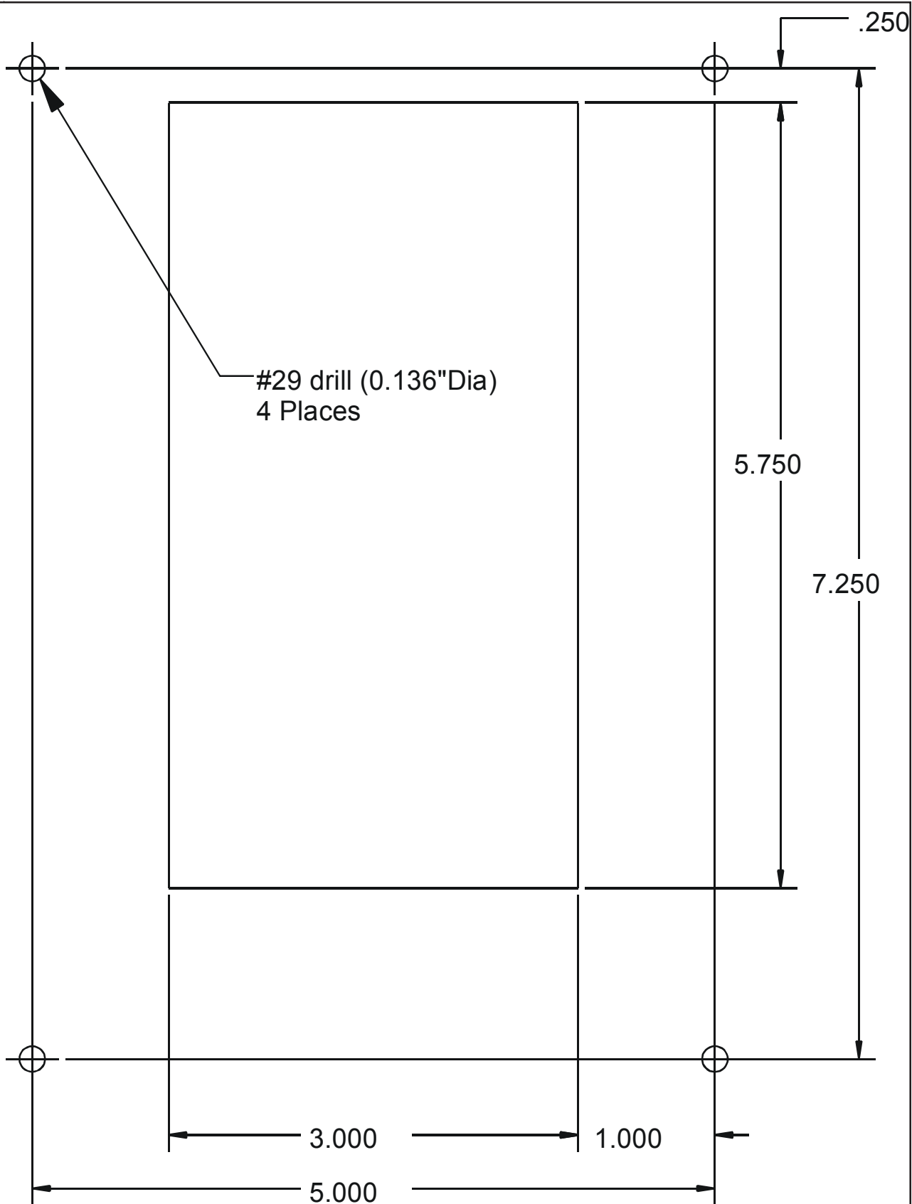
Figure 2 Hole Template
